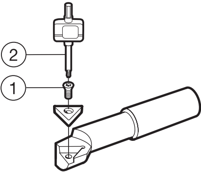
R429U-Axx..TC, R429U-E..TC
